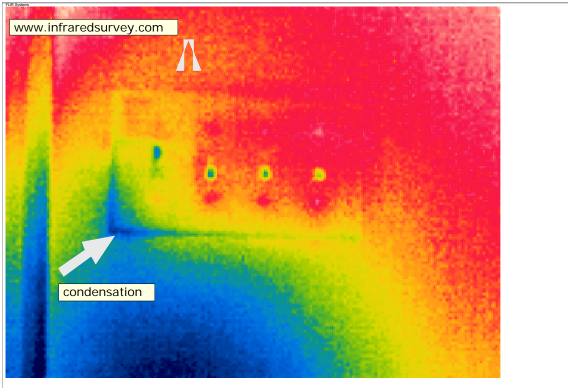
Description: Front door light switch with condensation evidence. Seal opening with gasket
