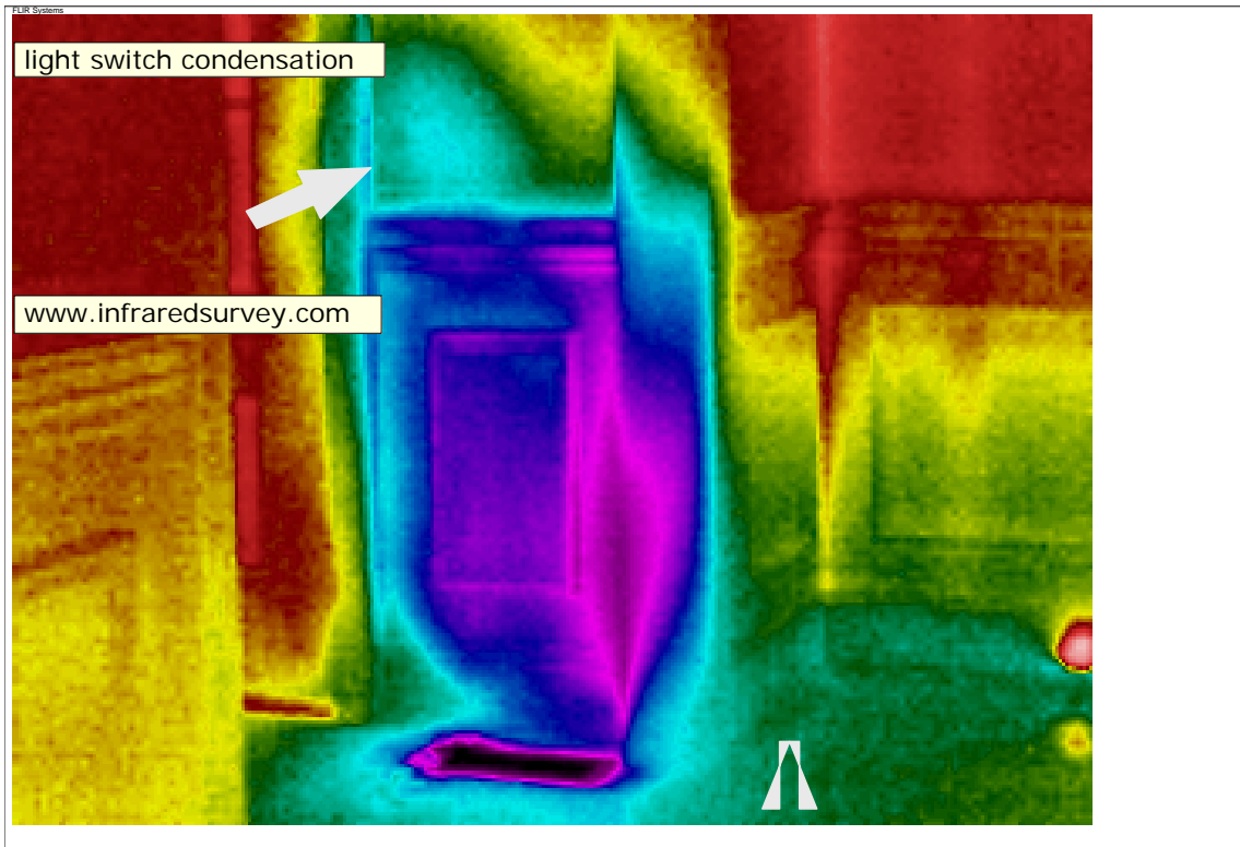
Description: Front door vent blowing on light switch with outside air leakage causing condensation
